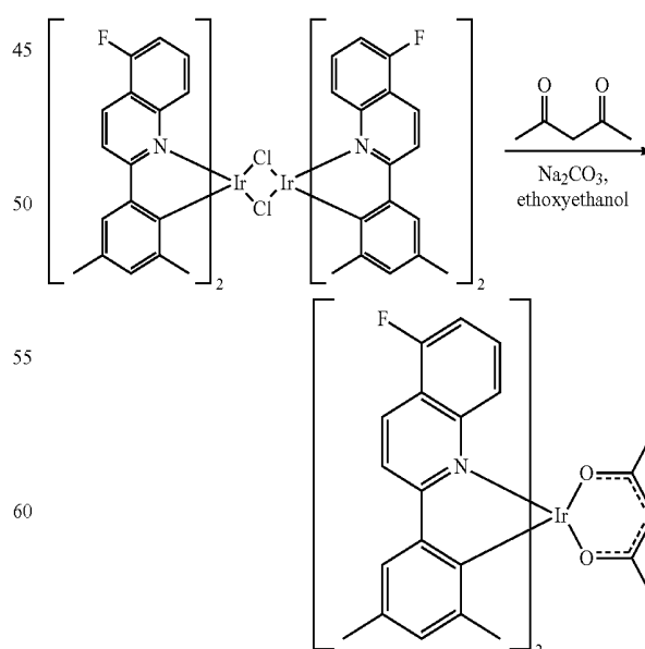
Compound 8
