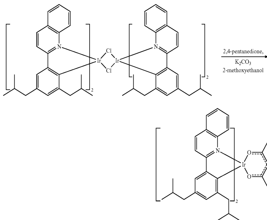
Compound 23
