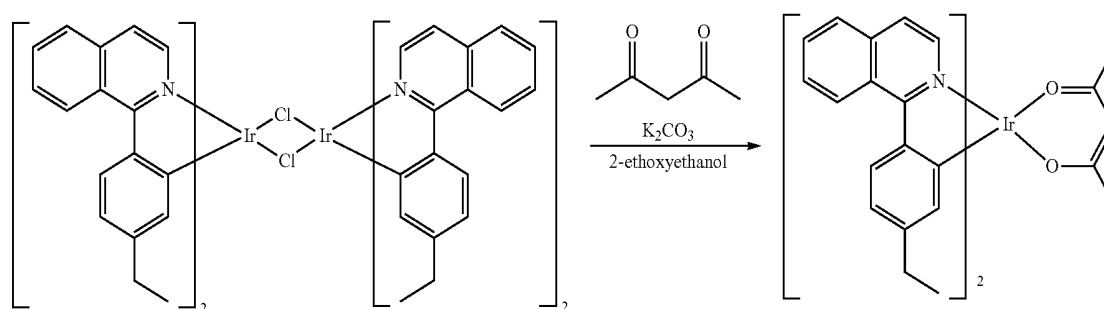
Compound 10
