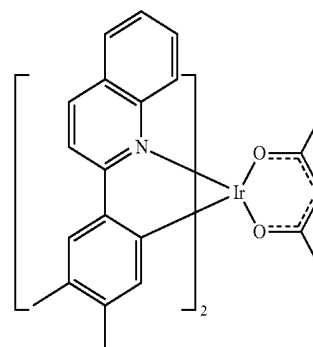
Compound 13
