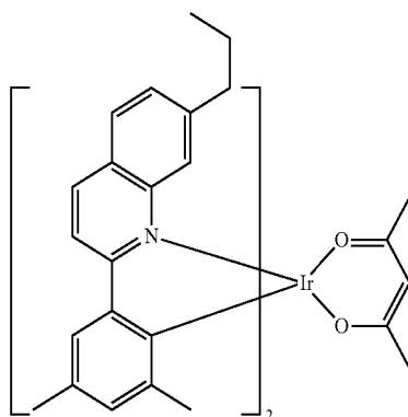
Compound 16
