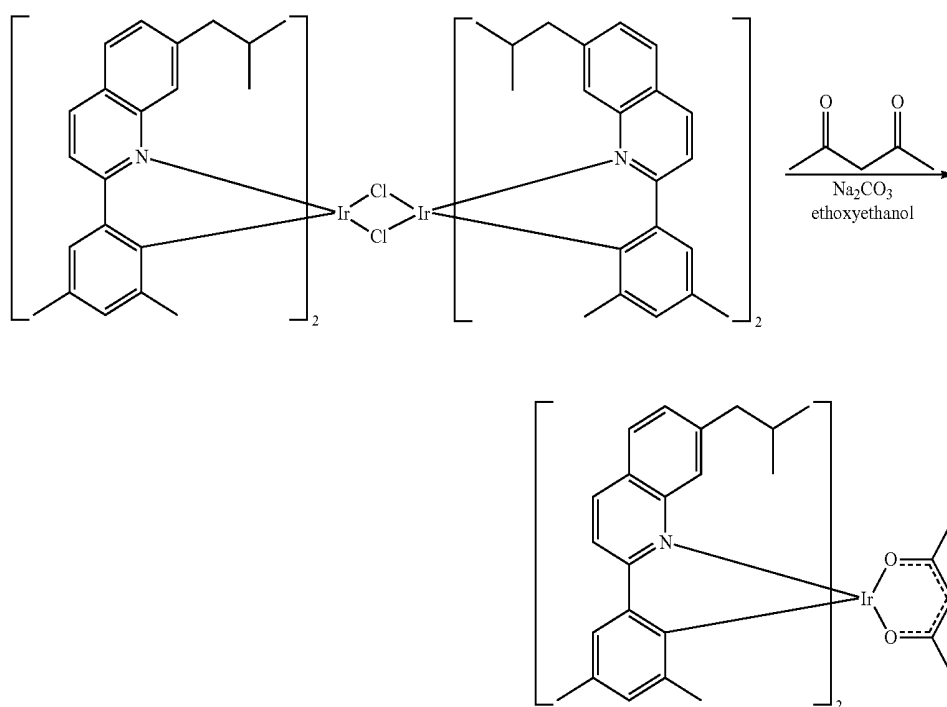
Compound 9
